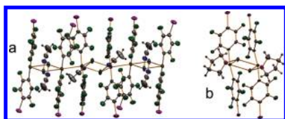
Figure 2. Structures of (a) polymeric 5 and (b) monomeric 4b motifs.
