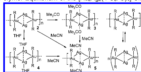
Scheme 1. (left) Vapochromic Reactions of 2–5 and (right) Dimer–Polymer Equilibrium of the [Au_2Ag_2(4-C_6F_4I)_4] Cluster
