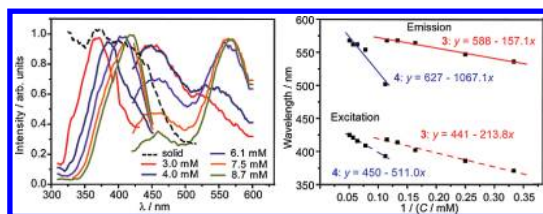
Figure 3. (left) Excitation and emission profiles of solid 3 and 3 in Me 2 CO at different concentrations. (right) Linear fits of the excitation and emission maxima of 3 (red) and 4 (blue) vs 1/C in Me 2 CO and THF, respectively.
