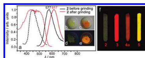
Figure 1. (a) Solid-state spectra and (b–e) mechanochromism of 2 (b, d) before and (c, e) after grinding (dashed line, absorption; solid line, emission). (f) Luminescence of excited 2 (before grinding), 3 , 4a , and 5 .
